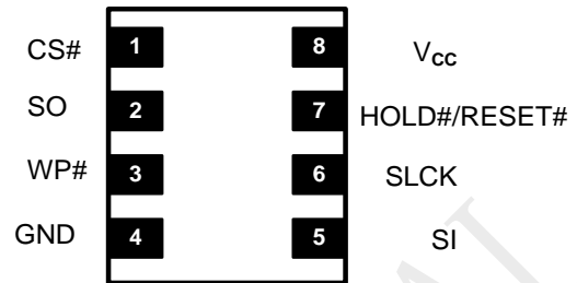
8-Land USON (1.5x1.5/3x2mm)
