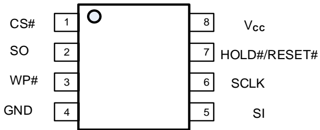
8-PIN SOP (150mil) and TSSOP
