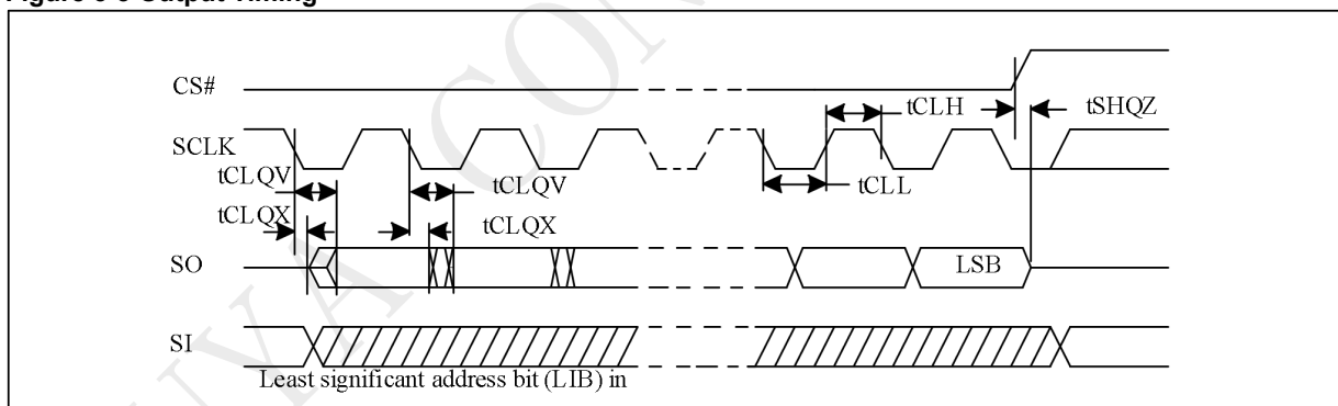
Figure 5-7 WP Timing
