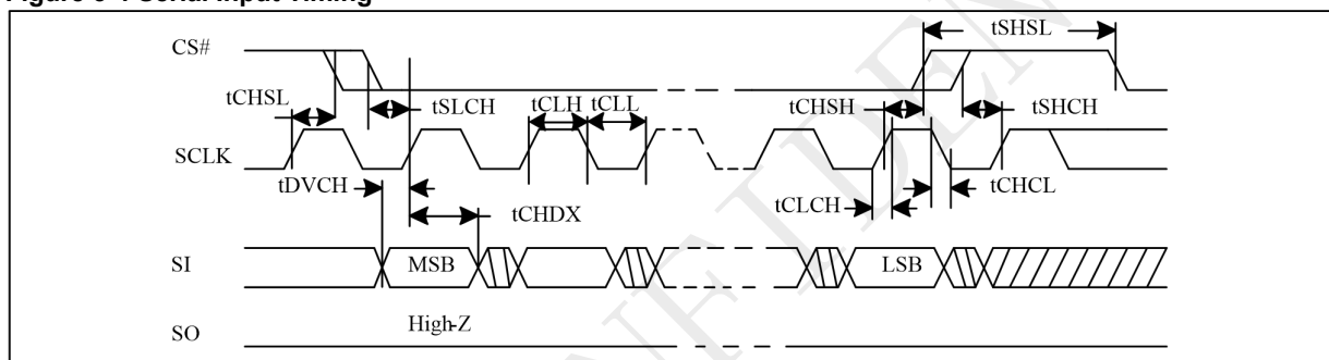
Figure 5-5 Output Timing
