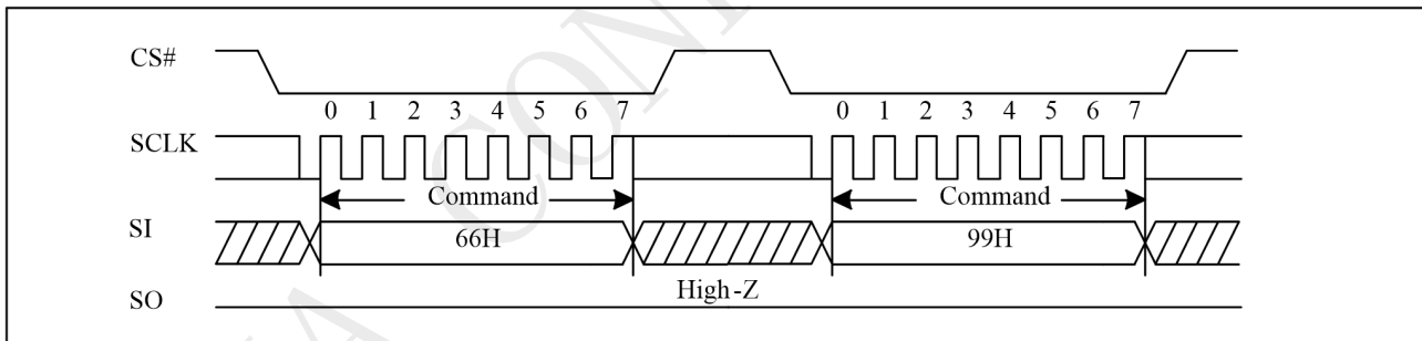
Figure 10-33a Reset Sequence
