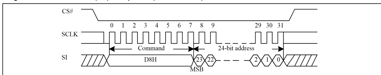
Figure 10-18 Block Erase (BE) Sequence (Command D8)
